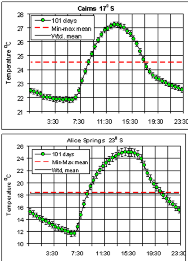
Figure 2: Temperatures measured at 30 minute intervals through a 24 hour day. The solid black line is the weighted average of readings every 30 minutes. The dashed red line is the average of the minimum and maximum temperatures
