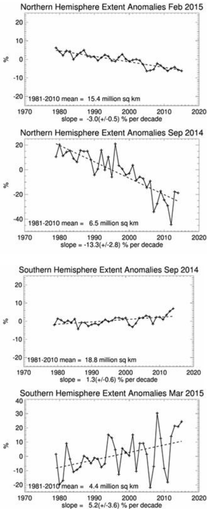
Figure 6: Arctic and Antarctica ice extent. The maximum extent occurs in February in the Northern Hemisphere and in September in the Southern Hemisphere. Summer minima occur in September and March. The Northern Hemisphere ice extent is decreasing with reducing
