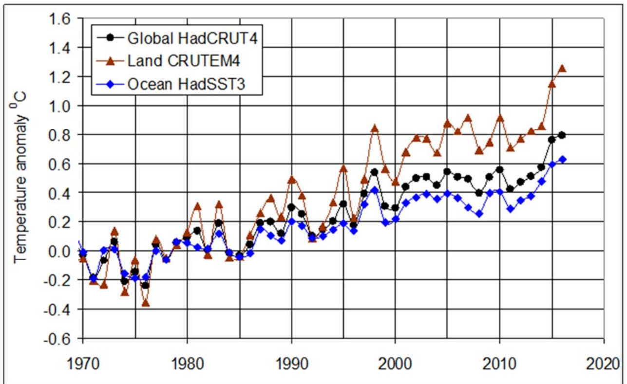
Figure 1: UK Met Office total, land and ocean global annual surface temperatures from 1970 to 2016 (an 11 month average).
