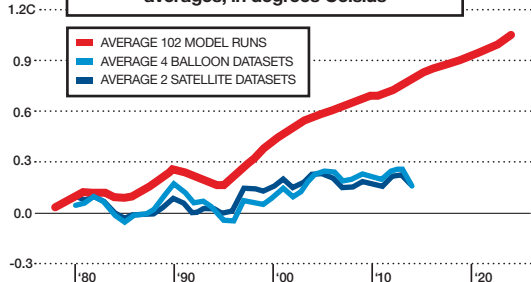
Global mid-tropospheric temperature 5-year averages, in degrees Celsius
